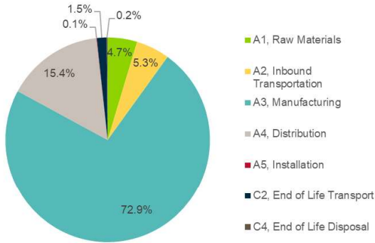
Global Warming Potential (kg CO 2 eq) by Stage for 1 m 2 Thermafiber® FF at R SI = 1 made in Wabash
