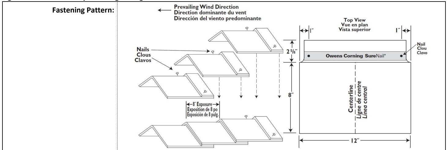
Figure 12 - Berkshire® Hip and Ridge Shingles
