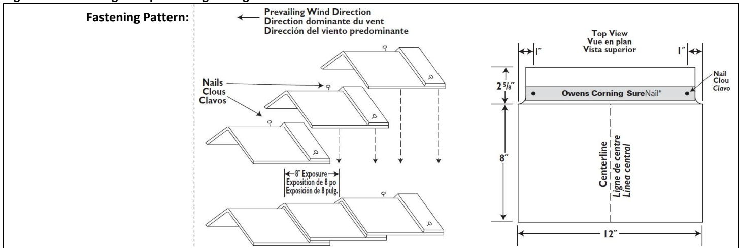
Figure 11 - DuraRidge™ Hip and Ridge Shingles
