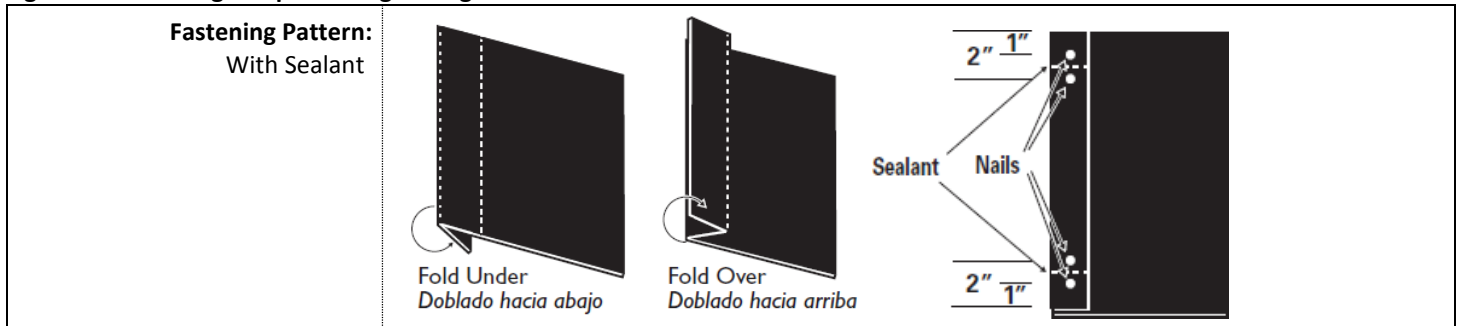
Figure 10 - RIZERidge® Hip and Ridge Shingles
