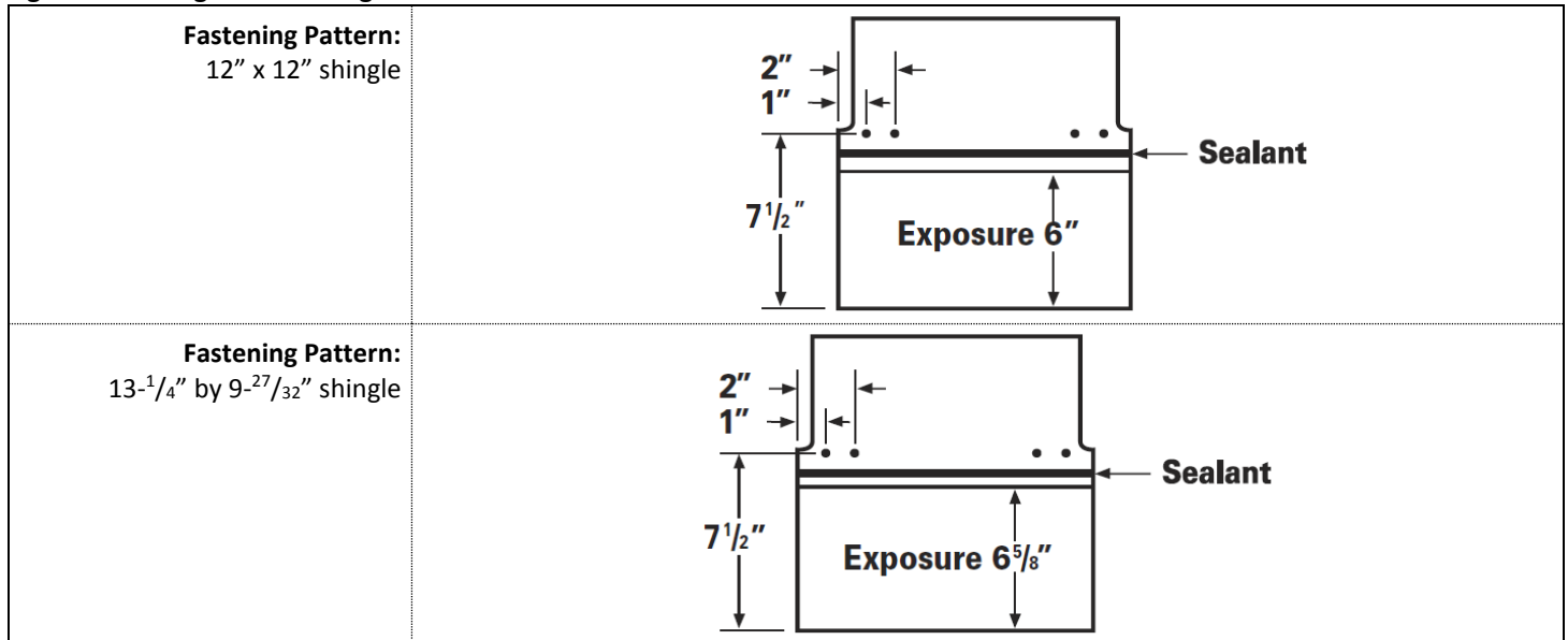
Figure 8 - ProEdge® and ProEdge® FLEX™
