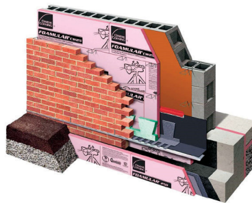
The CavityComplete ® Concrete Masonry Unit (CMU) Wall System excludes the masonry veneer and concrete masonry units. A detailed list of the components is available at www.CavityComplete.com .
