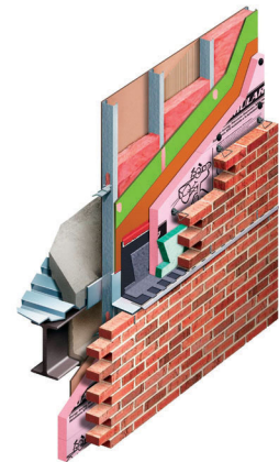
The CavityComplete ® Wall System excludes the masonry veneer, steel studs and interior and exterior gypsum board. A detailed list of the components is available at www.CavityComplete.com .
