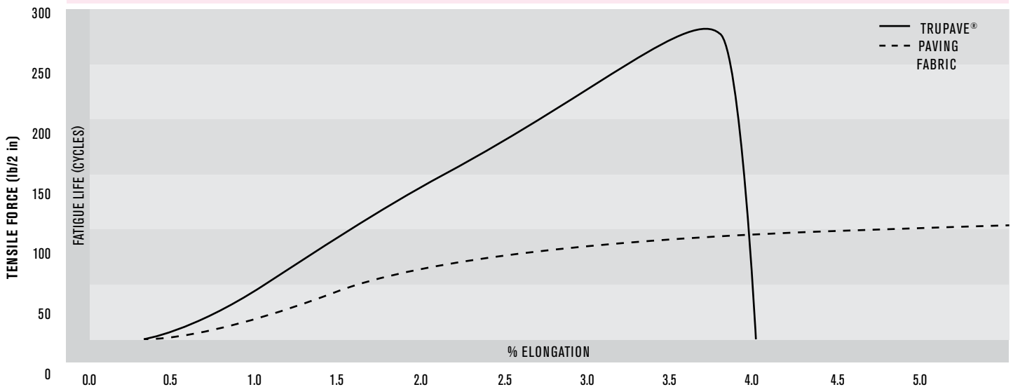
COMPARISON OF TRUPAVE® AND PAVING FABRICS IN ASPHALT: TENSILE STRENGTH
